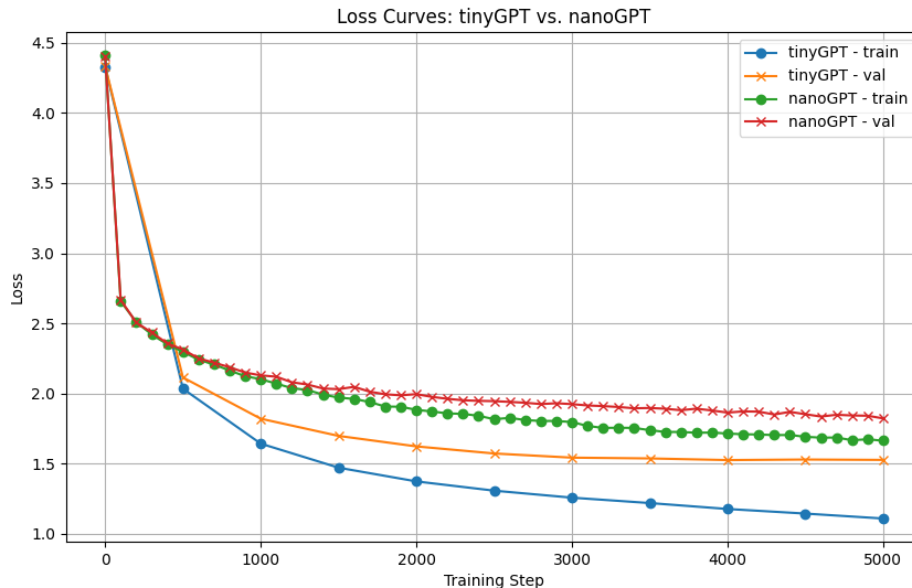
Figure 2: Loss curves on same dataset and similar size models.
